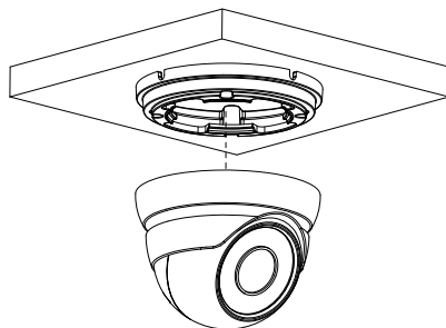
Figure 3-4 Installing and adjusting camera
