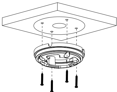
Figure 3-3 Install the camera base
